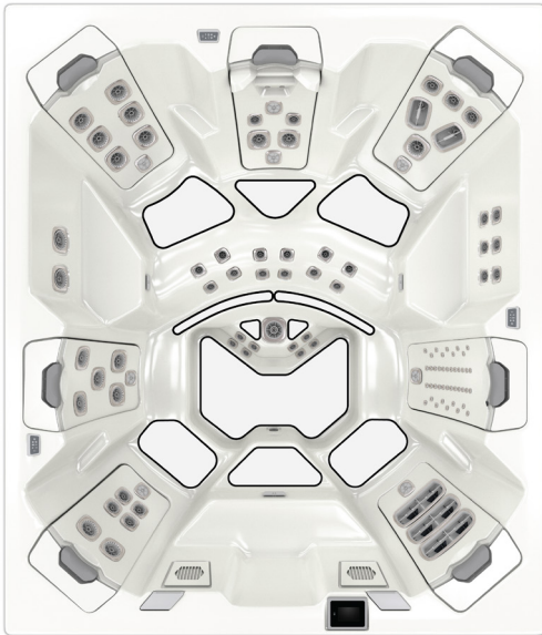
M7 Non-slip Aquatic Surface Layout
